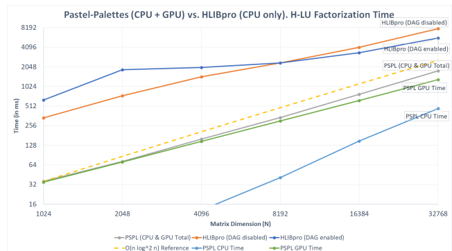
Figure 3: Pastel-Palettes vs. HLIBpro. H-LU Performance.
